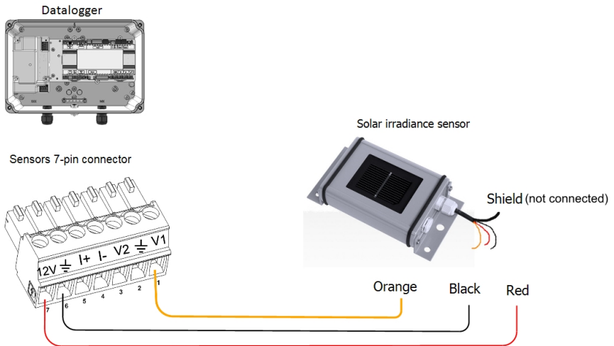
Figure 18: Solar irradiance sensor connection
