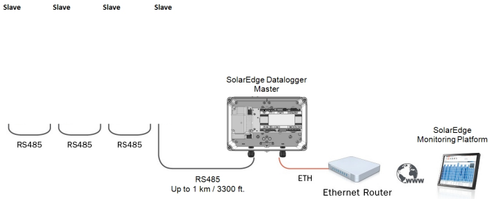
Figure 4: Example of RS485 connection
