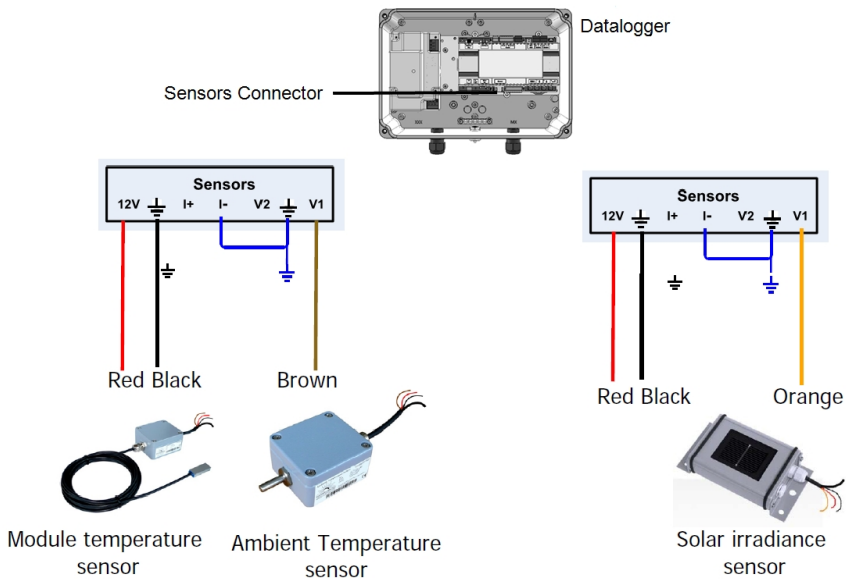
Figure 17: Sensors connection diagram
